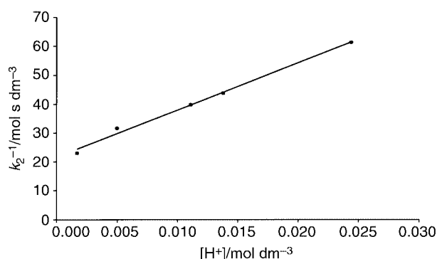
Fig. 3 Plot of 1/k_2 vs. [H^+] for the oxidation of phosphite by [Ru^{VI}(L)(O)_2]^{2+} at T = 298.0 K and I = 0.2 mol dm -3 .
