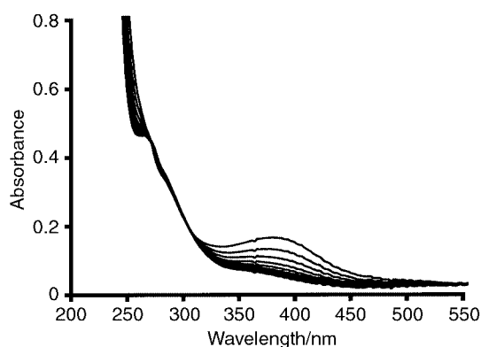
Fig. 1 Spectral changes during the oxidation of excess hypophosphite ( 1 \times 10^{-3} \text{ mol dm}^{-3} ) by \text{trans-[Ru}^{\text{VI}}(\text{L})(\text{O})_2]^{2+} ( 1 \times 10^{-4} \text{ mol dm}^{-4} ) at T = 298.0 \text{ K} , I = 1.0 \text{ mol dm}^{-3} and \text{pH} = 1.9 . Path length b = 1.0 \text{ cm} . Time between consecutive runs = 60 s.
