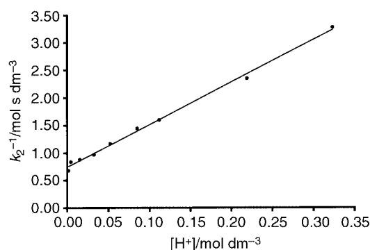
Fig. 2 Plot of 1/k_2 vs. [\text{H}^+] for the oxidation of hypophosphite by \text{trans-[Ru}^{\text{VI}}(\text{L})(\text{O})_2]^{2+} at T = 298.0 \text{ K} and I = 1.0 \text{ mol dm}^{-3} .
